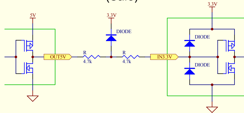
Conventional CMOS device with protection diodes
