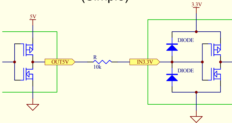
Conventional CMOS device with protection diodes
