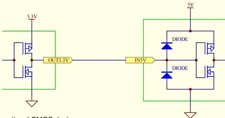
Conventional CMOS device ( V_{ol}=0V/V_{oh}=3.3V full swing)
